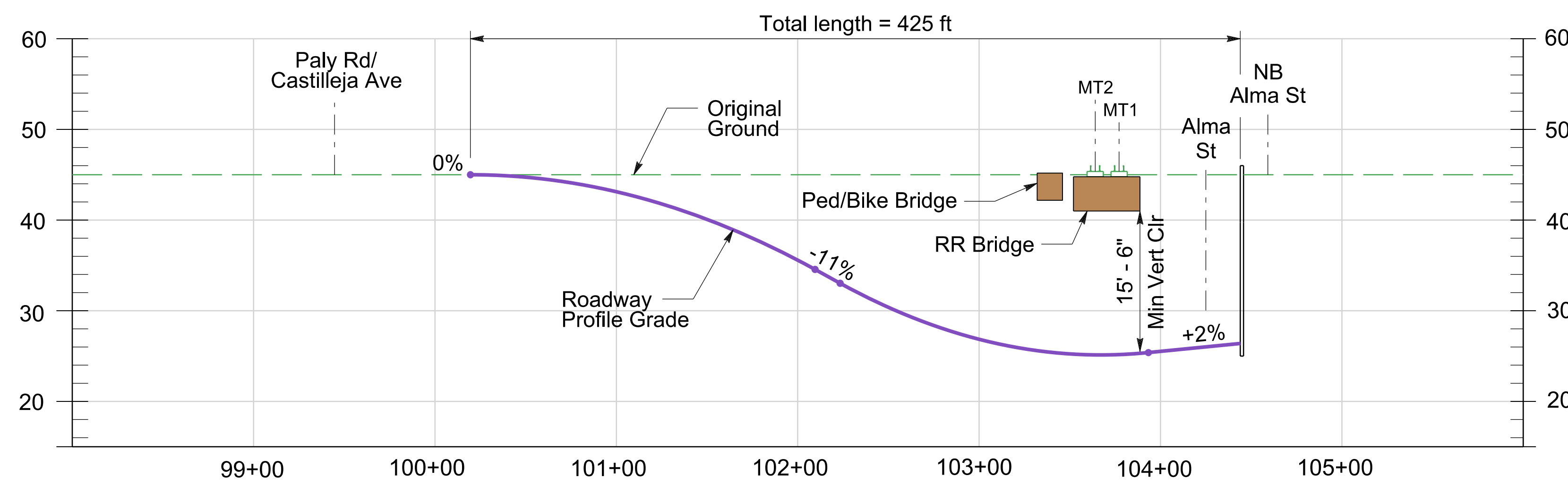
Churchill Ave (Profile)
