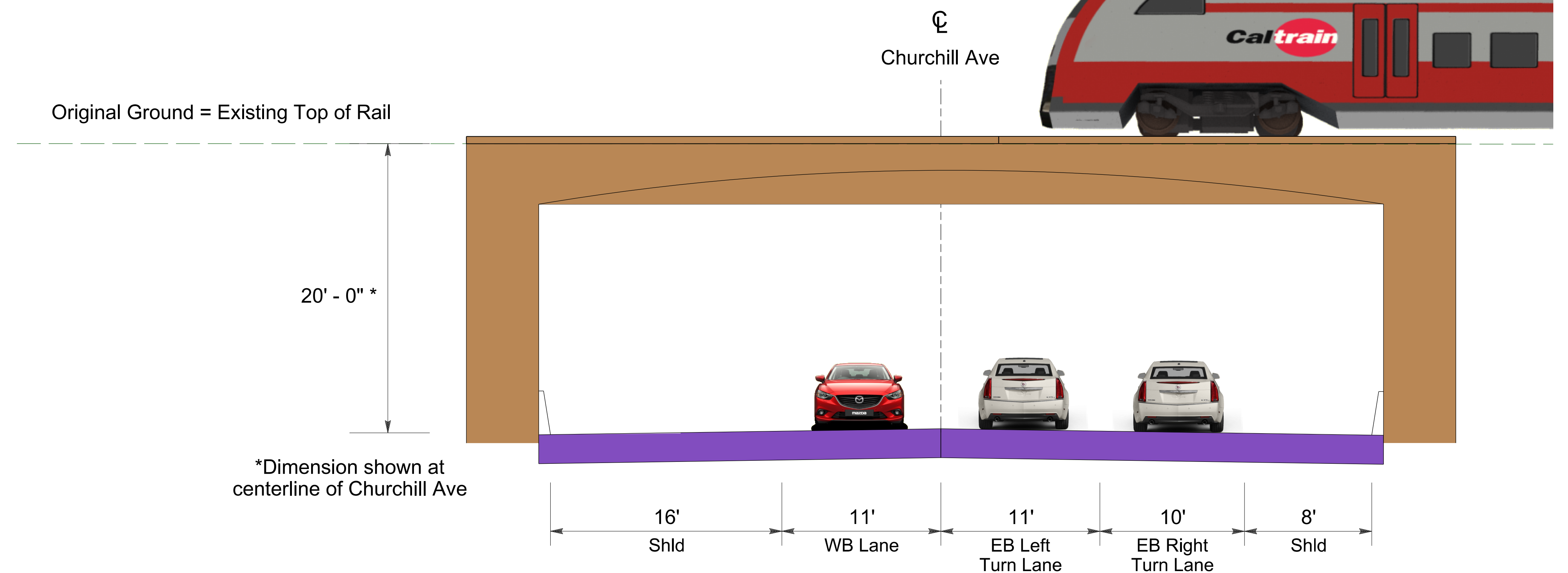
Typical Section Churchill Ave Underpass
