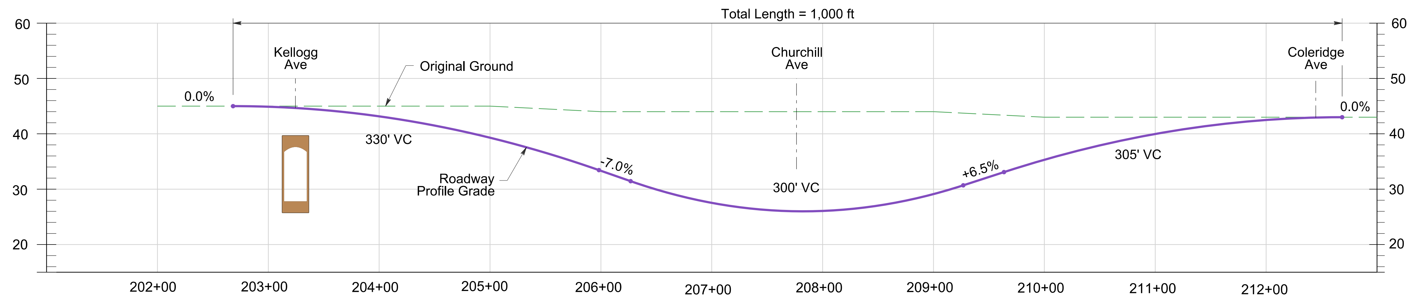
Alma St (Profile)
