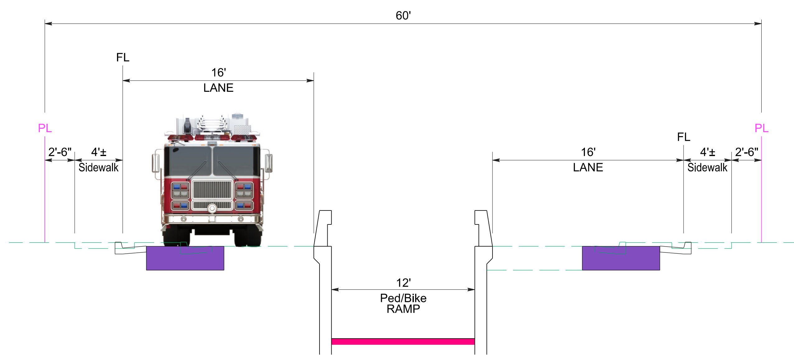
Typical Section Kellogg Ave
